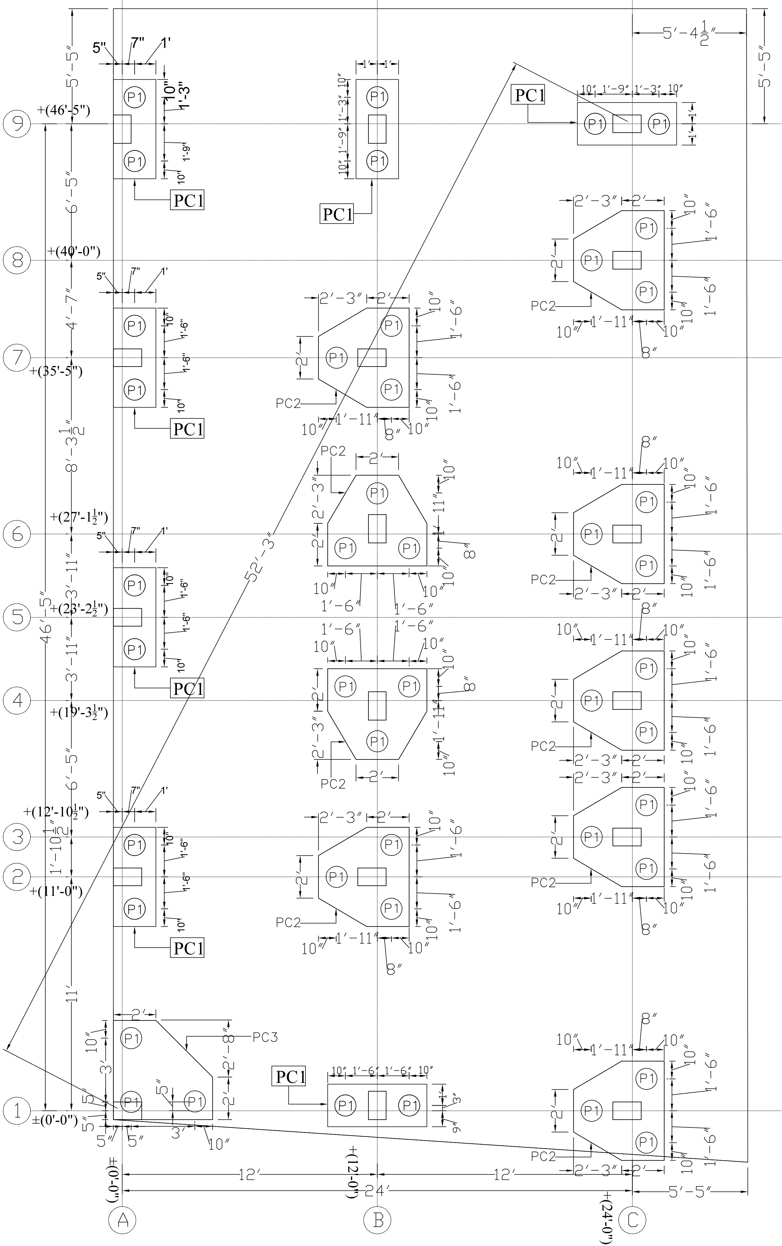
FOUNDATION LAYOUT PLAN
