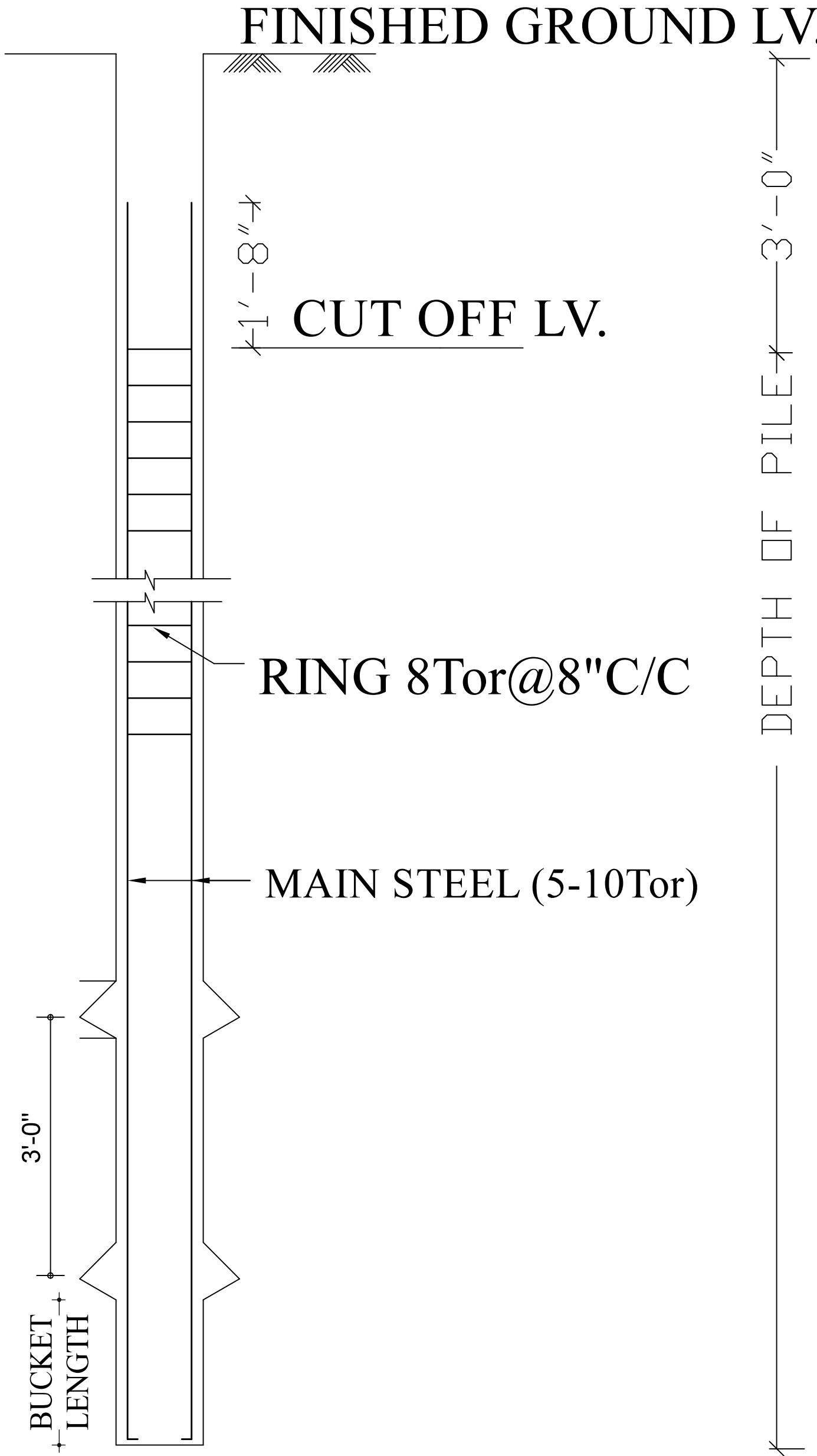
TYPICAL DETAILS OF UNDER REAMED PILE
